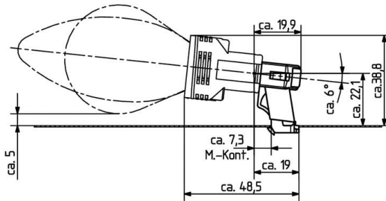
Adaptor combined with lampholder
